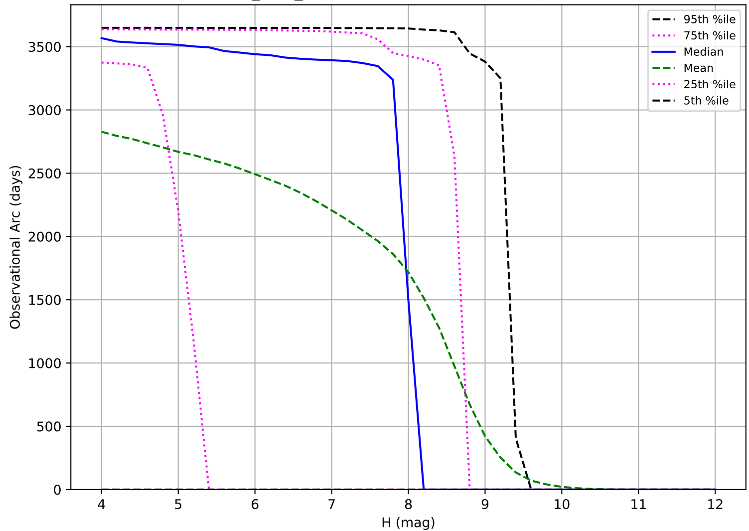
octo_v3.4_10yrs: Observational Arc Length TNO
