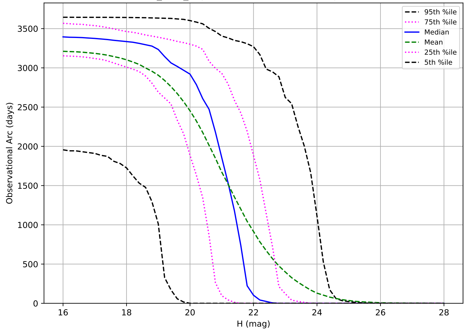
octo_v3.4_10yrs: Observational Arc Length PHA
