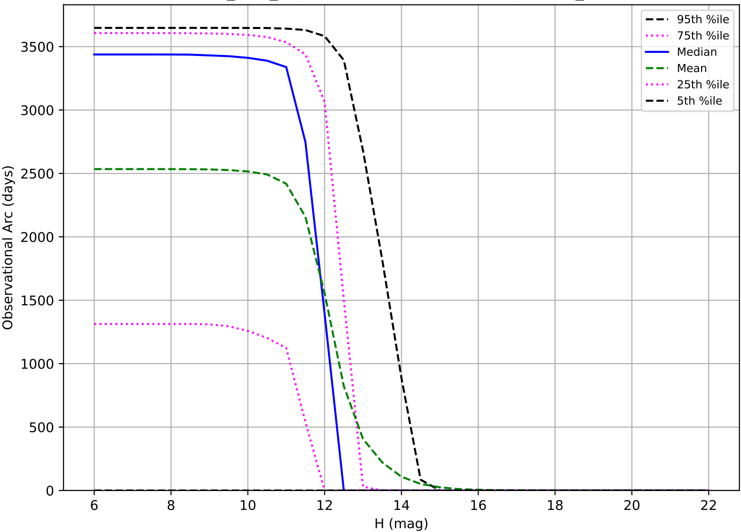
octo_v3.4_10yrs: Observational Arc Length OCC_r20
