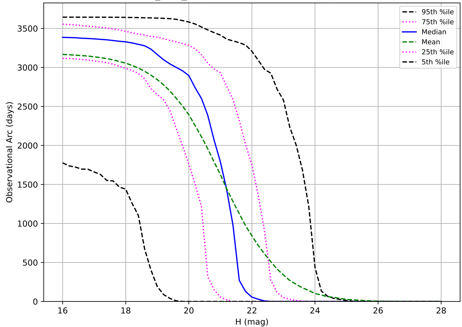
octo_v3.4_10yrs: Observational Arc Length NEO
