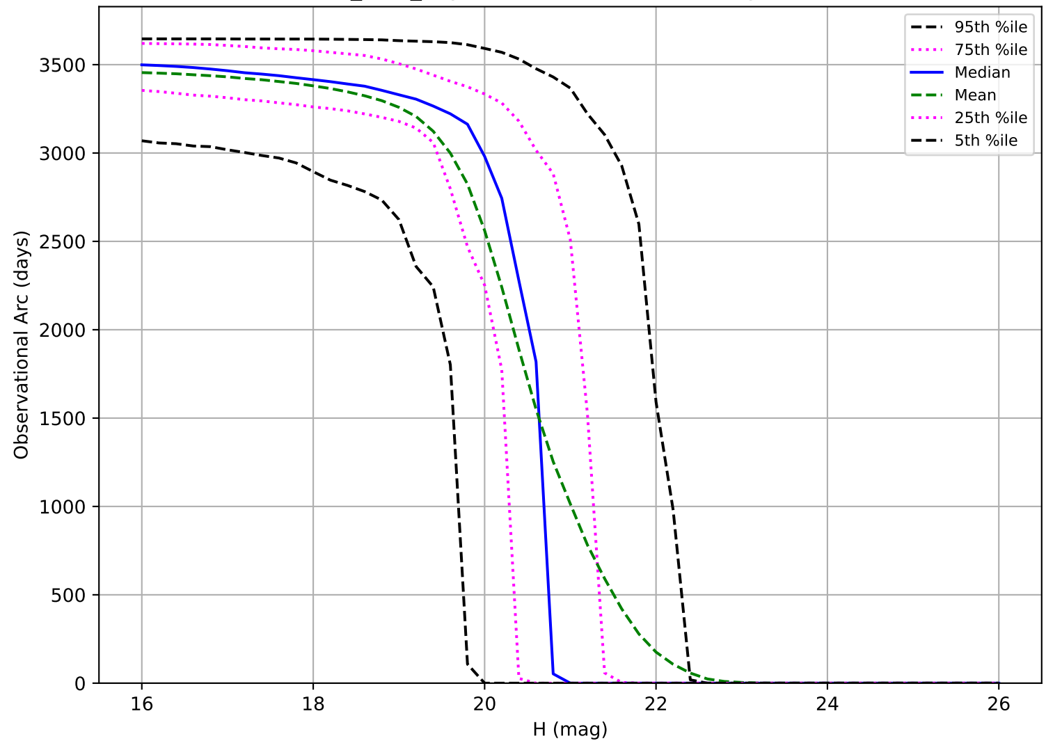
octo_v3.4_10yrs: Observational Arc Length MBA
