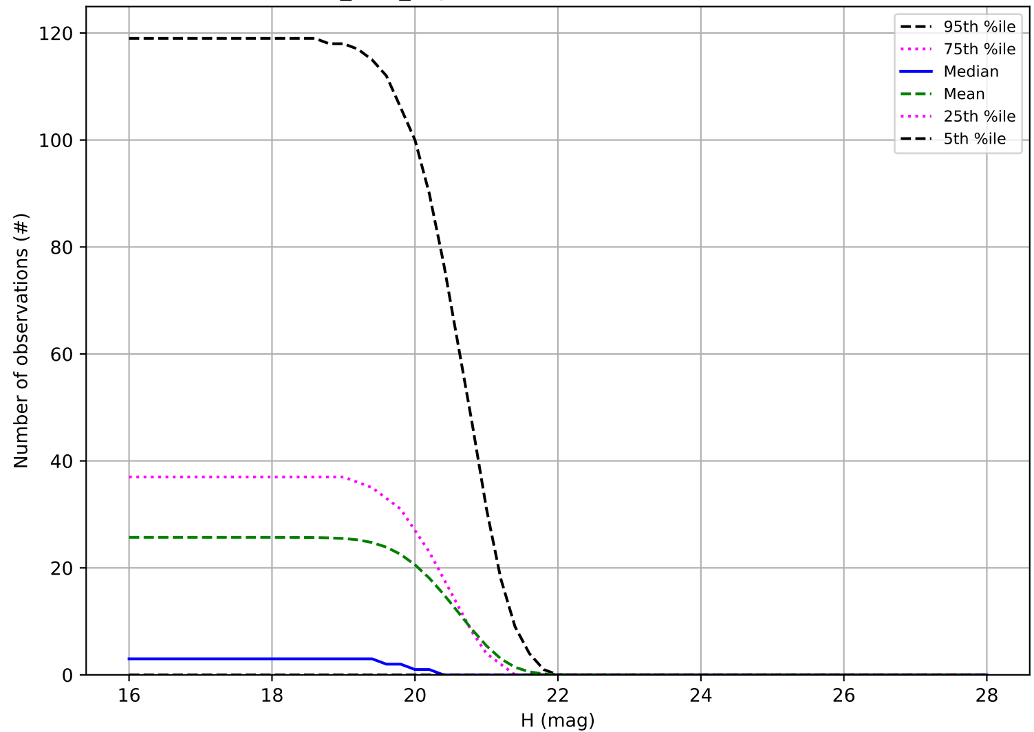
octo_v3.4_10yrs: Number of observations Vatira
