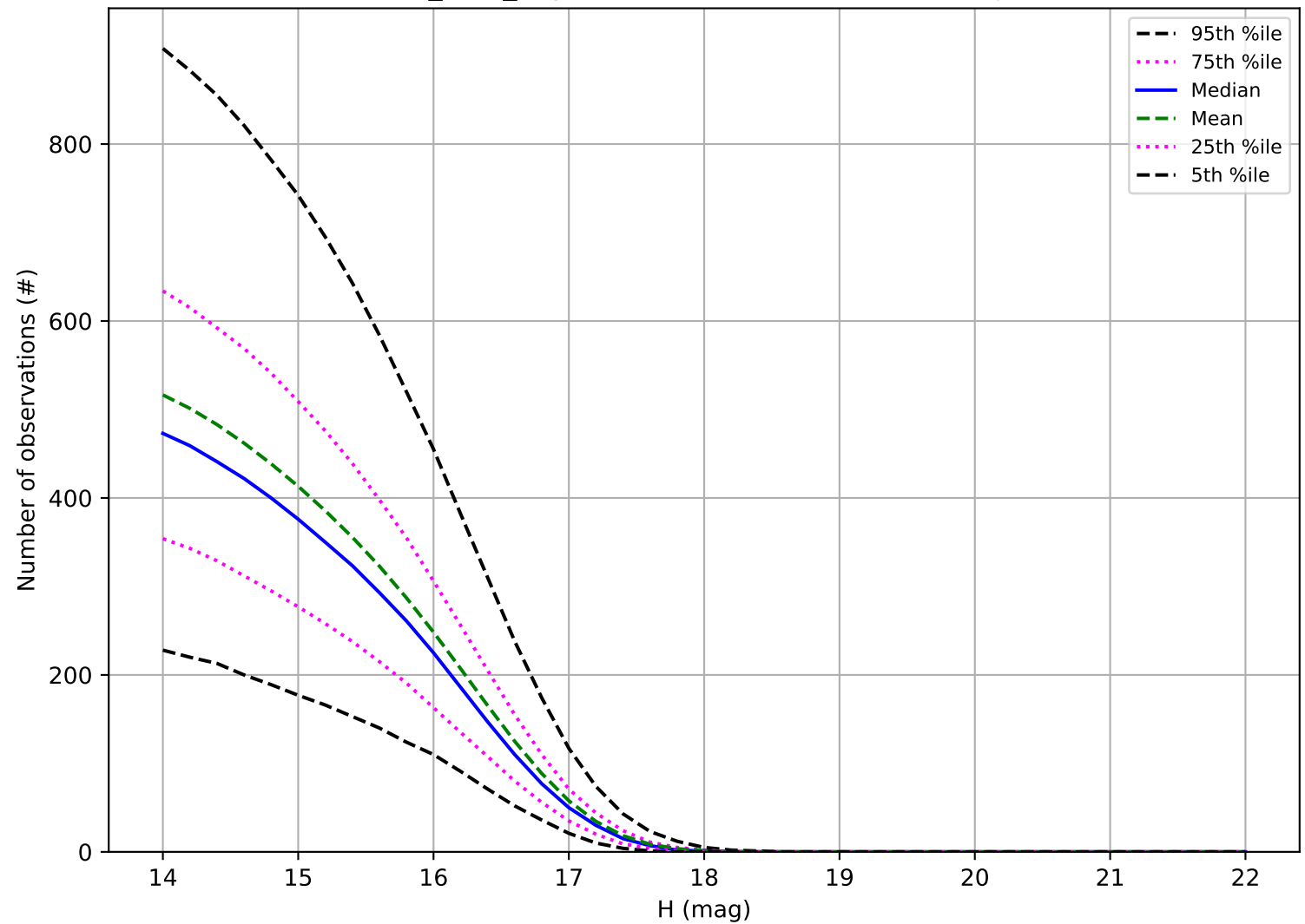
octo_v3.4_10yrs: Number of observations Trojan
