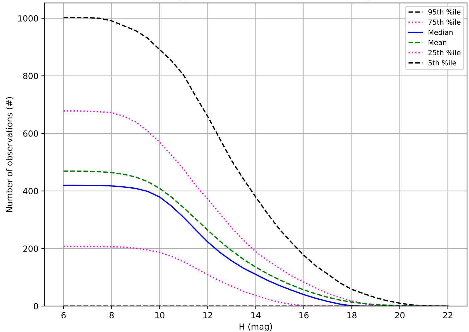
octo_v3.4_10yrs: Number of observations OCC_r5
