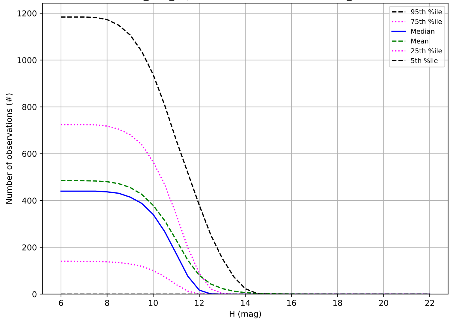
octo_v3.4_10yrs: Number of observations OCC_r20
