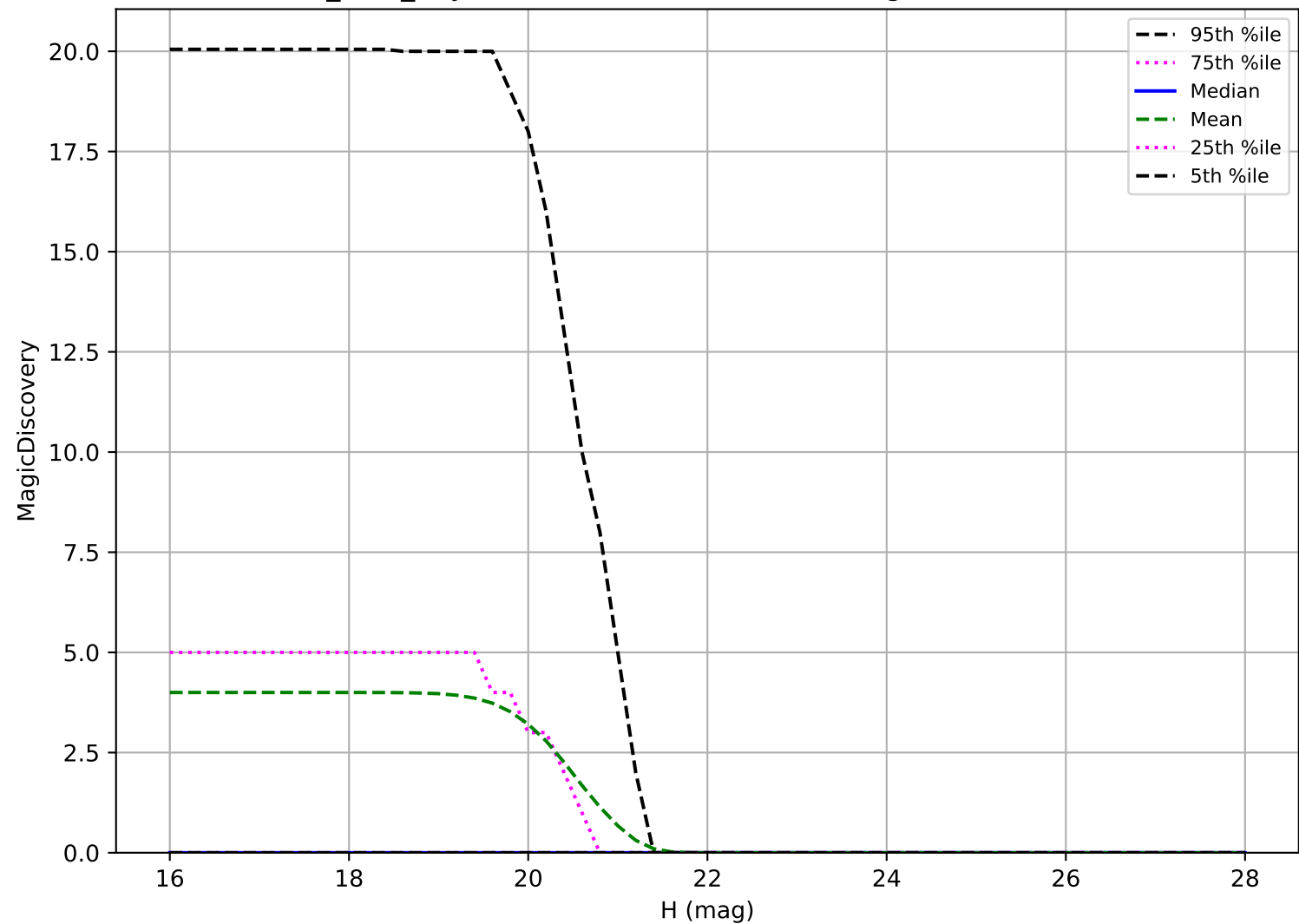
octo_v3.4_10yrs: Vatira 6 detections in 60 nights detection loss
