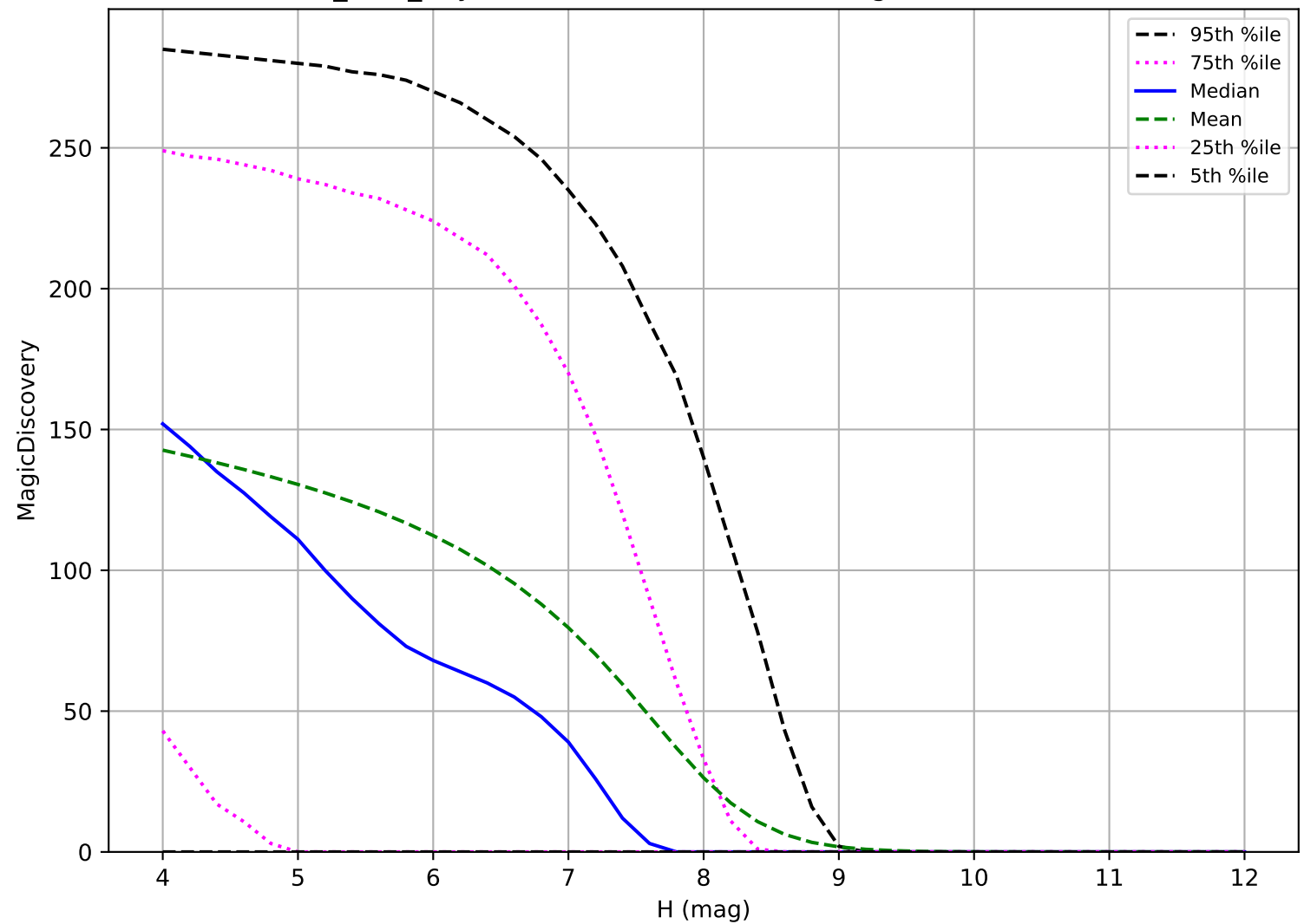
octo_v3.4_10yrs: TNO 6 detections in 60 nights detection loss
