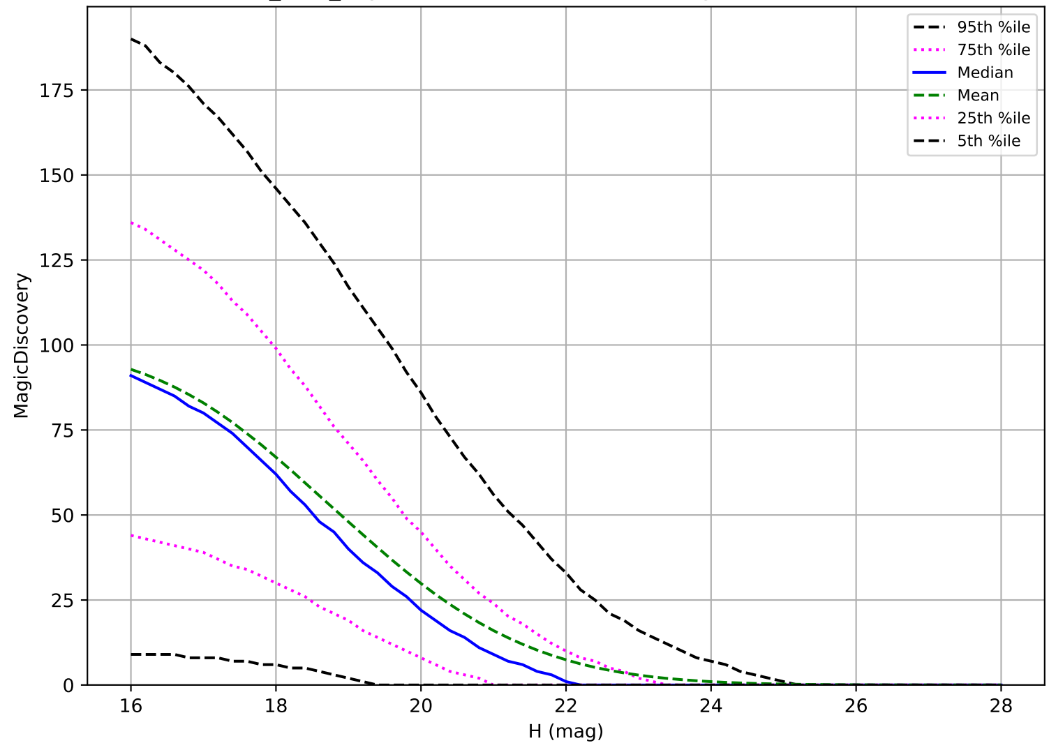
octo_v3.4_10yrs: PHA 6 detections in 60 nights detection loss
