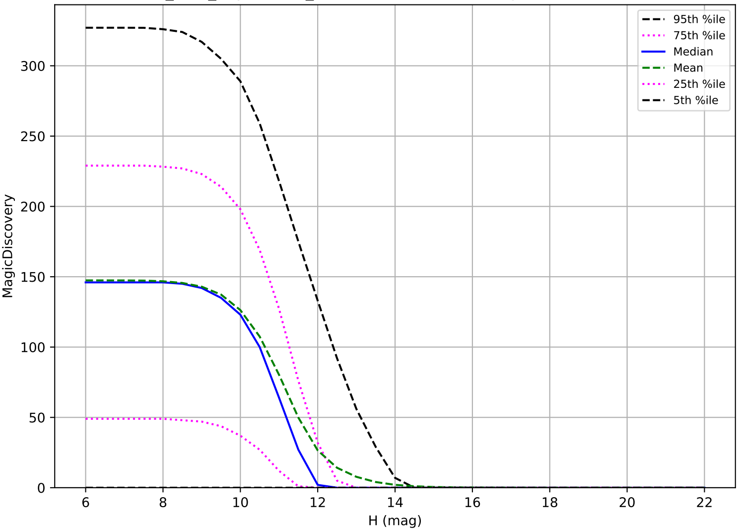
octo_v3.4_10yrs: OCC_r20 6 detections in 60 nights detection loss
