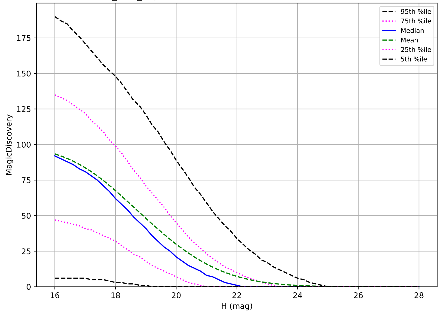
octo_v3.4_10yrs: NEO 6 detections in 60 nights detection loss
