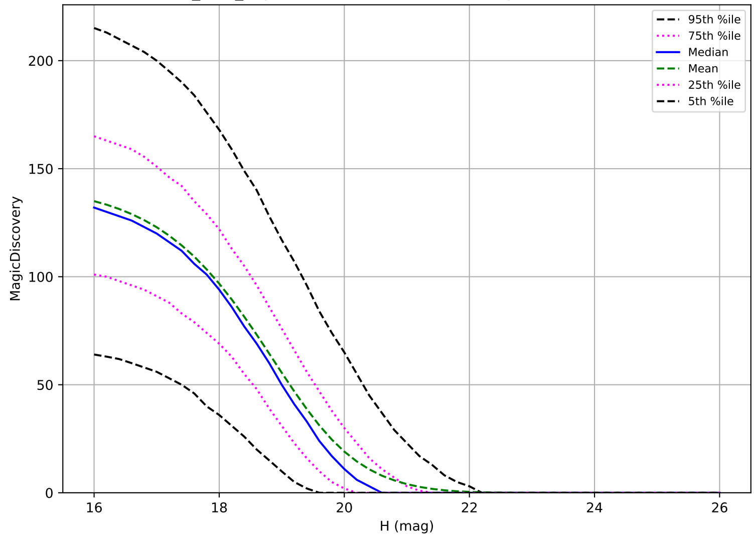
octo_v3.4_10yrs: MBA 6 detections in 60 nights detection loss
