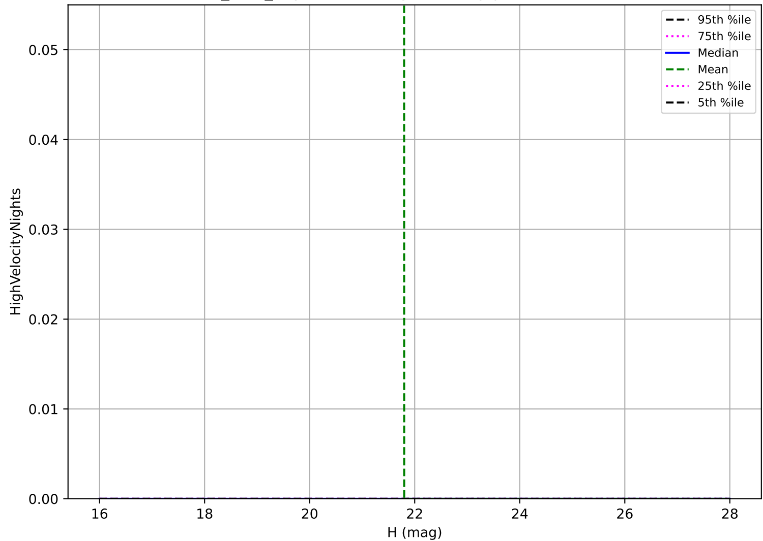
octo_v3.4_10yrs: Vatira High velocity pair detection loss
