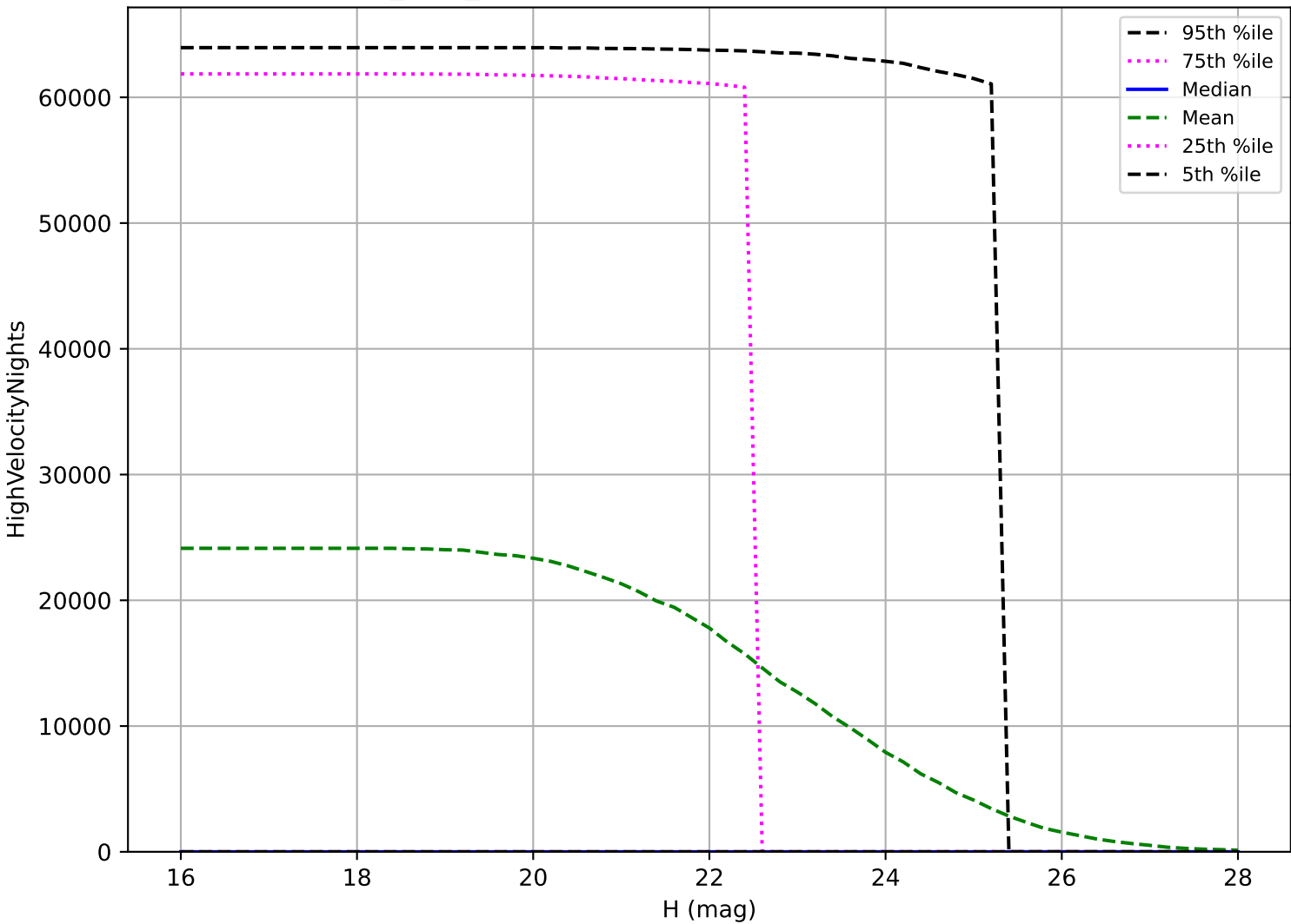
octo_v3.4_10yrs: PHA High velocity pair detection loss
