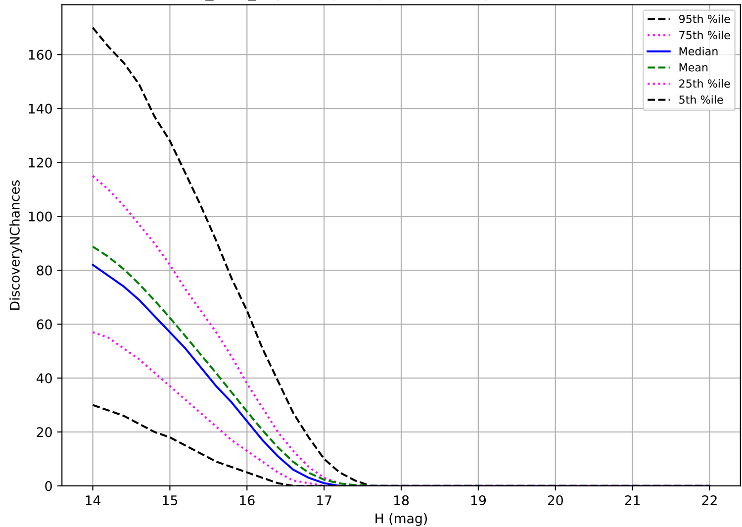
octo_v3.4_10yrs: Trojan 3 pairs in 15 nights detection loss
