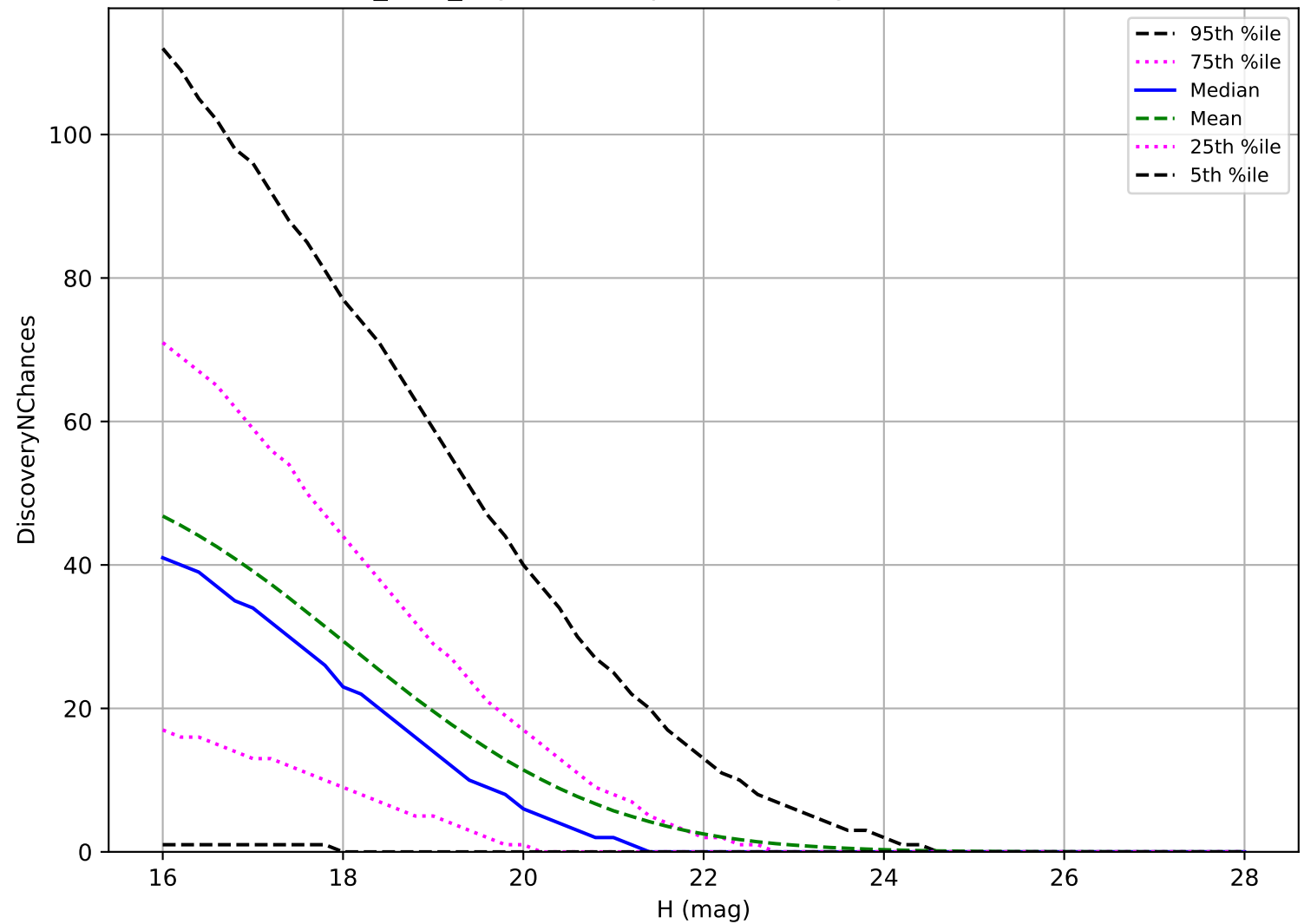
octo_v3.4_10yrs: PHA 3 pairs in 15 nights detection loss
