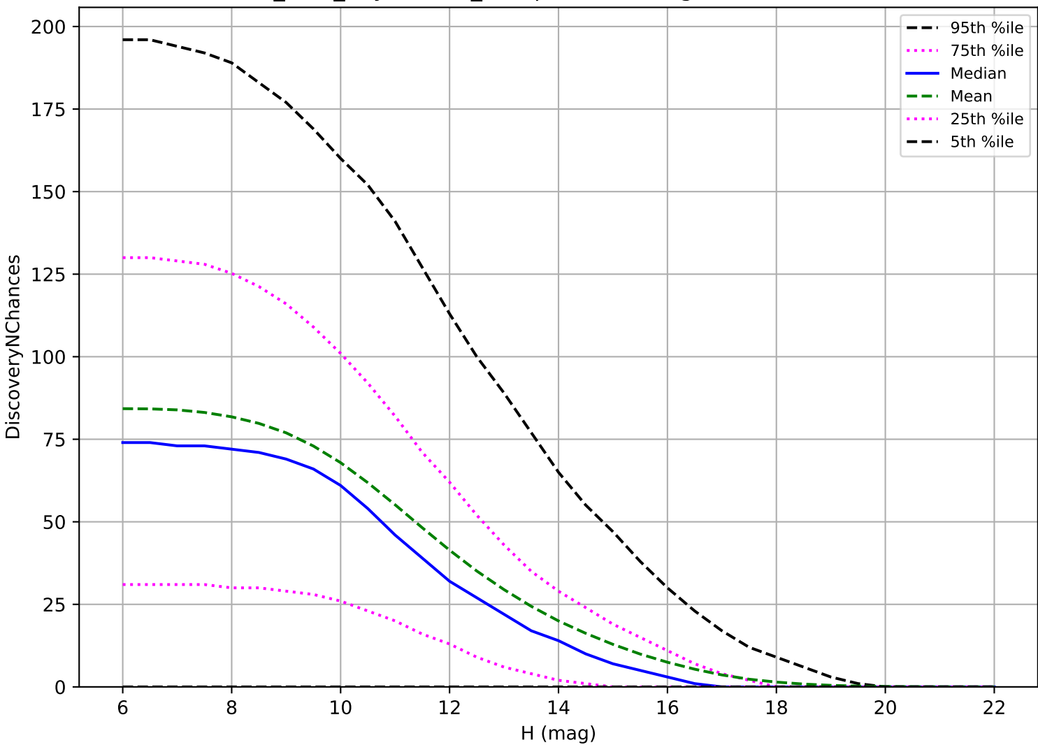
octo_v3.4_10yrs: OCC_r5 3 pairs in 15 nights detection loss
