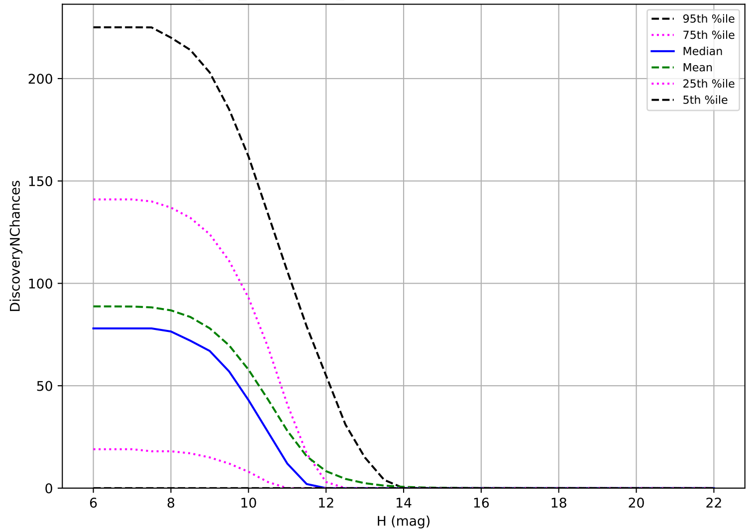
octo_v3.4_10yrs: OCC_r20 3 pairs in 15 nights detection loss
