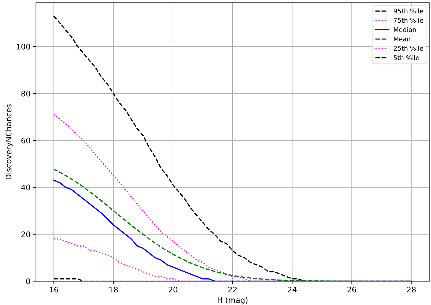
octo_v3.4_10yrs: NEO 3 pairs in 15 nights detection loss
