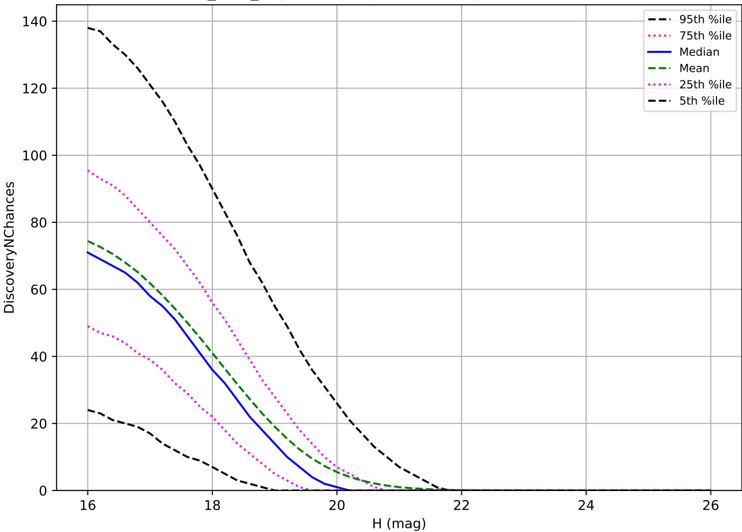
octo_v3.4_10yrs: MBA 3 pairs in 15 nights detection loss
