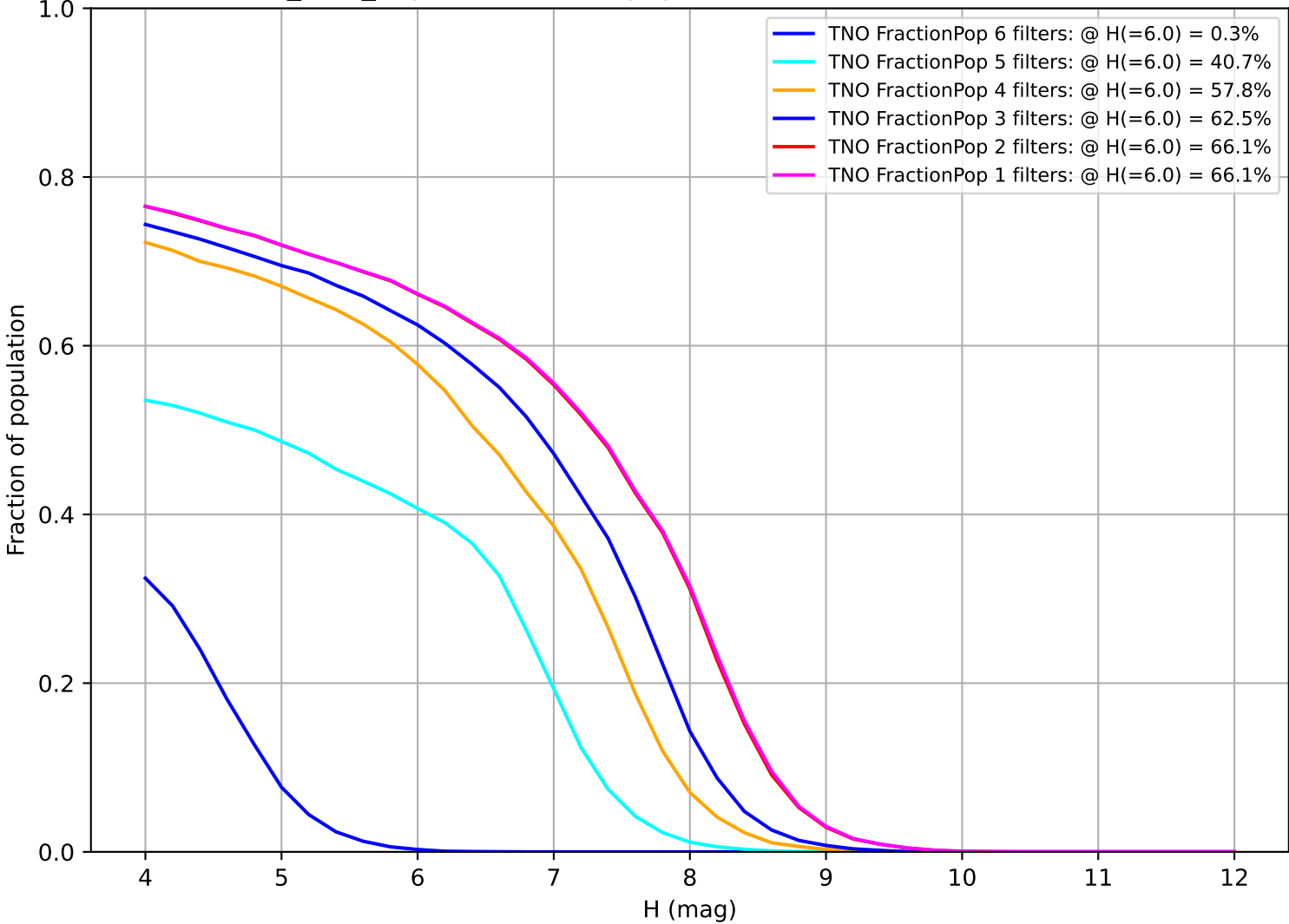
octo_v3.4_10yrs: Fraction of population with colors in X filters TNO
