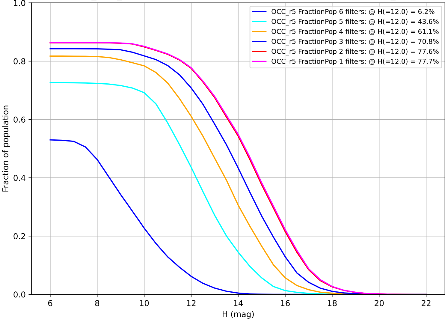
octo_v3.4_10yrs: Fraction of population with colors in X filters OCC_r5
