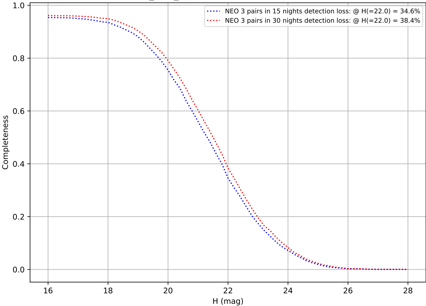
octo_v3.4_10yrs: DifferentialCompleteness
