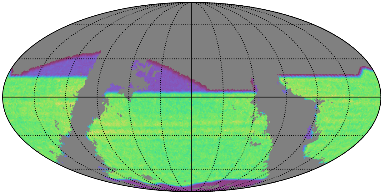
octo_v3.4_10yrs gri band non-DD: riz_exposure_time_year9
