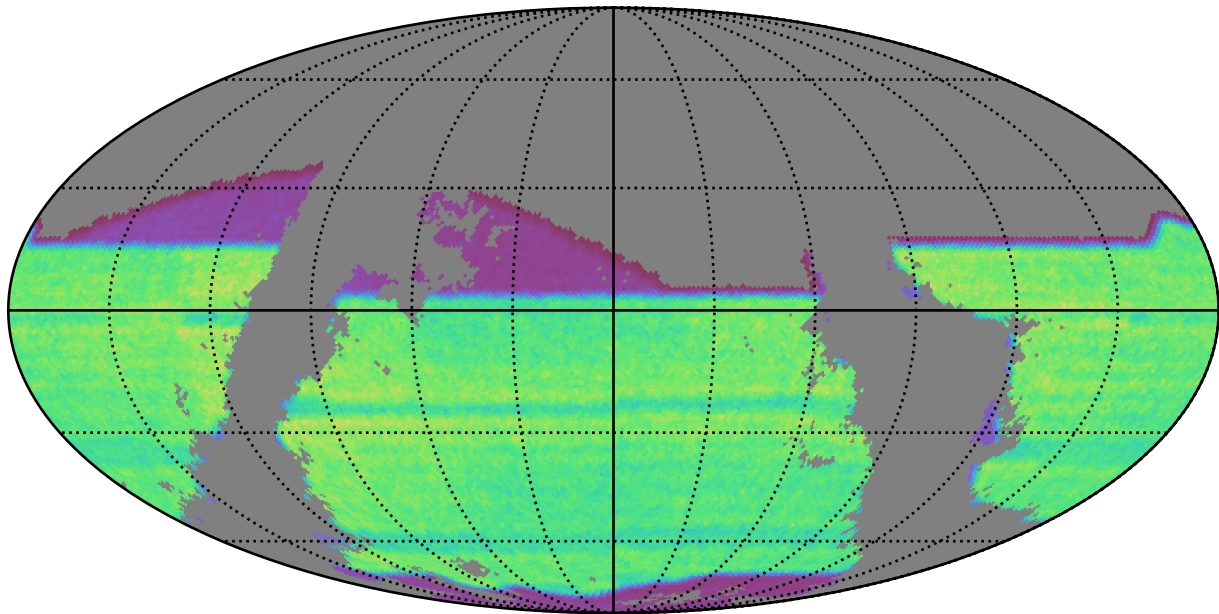
octo_v3.4_10yrs gri band non-DD: riz_exposure_time_year8
