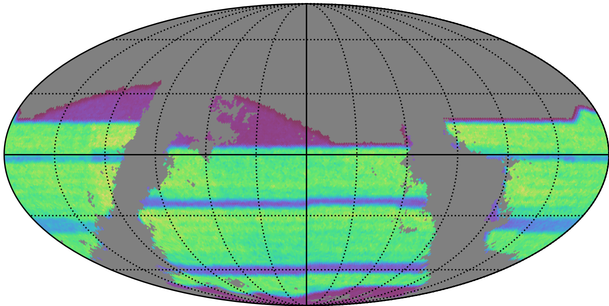
octo_v3.4_10yrs gri band non-DD: riz_exposure_time_year7
