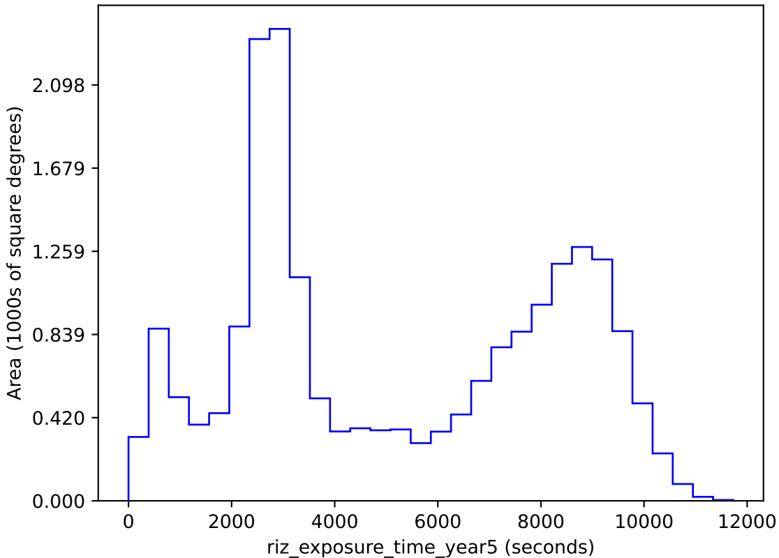
octo_v3.4_10yrs gri band non-DD: riz_exposure_time_year5
