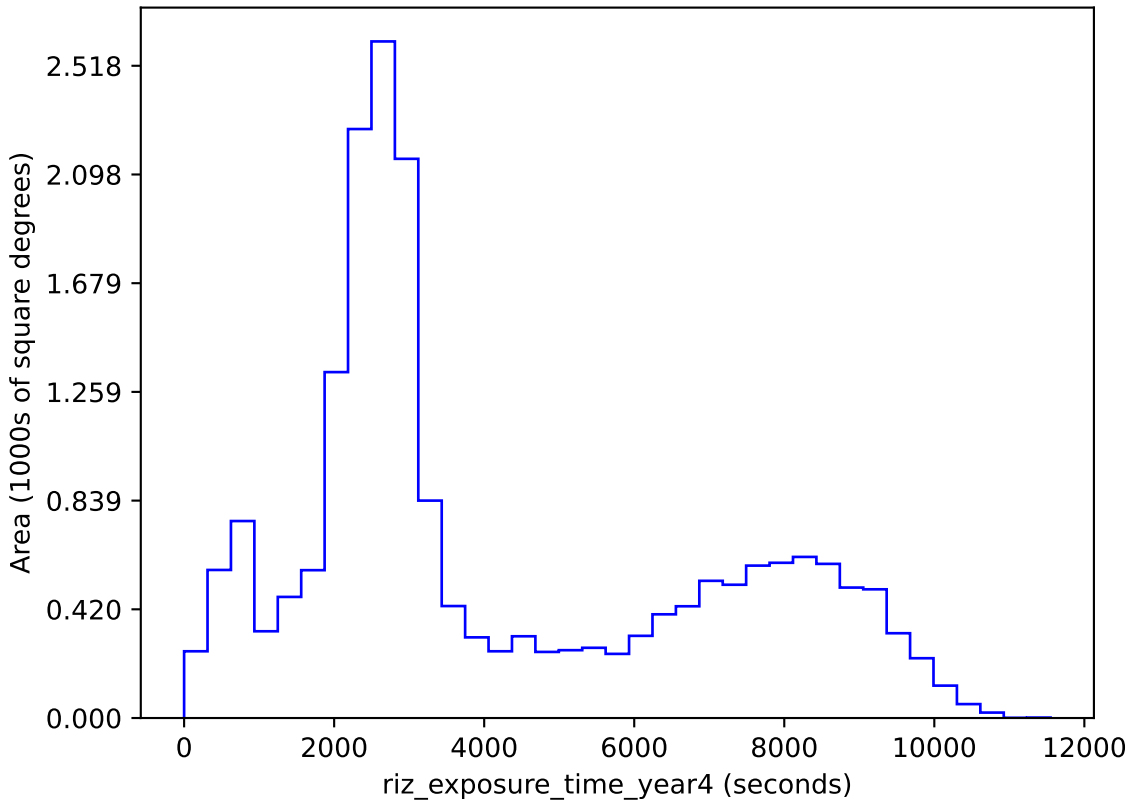
octo_v3.4_10yrs gri band non-DD: riz_exposure_time_year4
