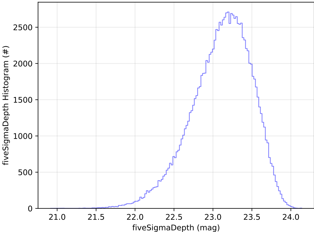
octo_v3.4_10yrs u: fiveSigmaDepth Histogram
