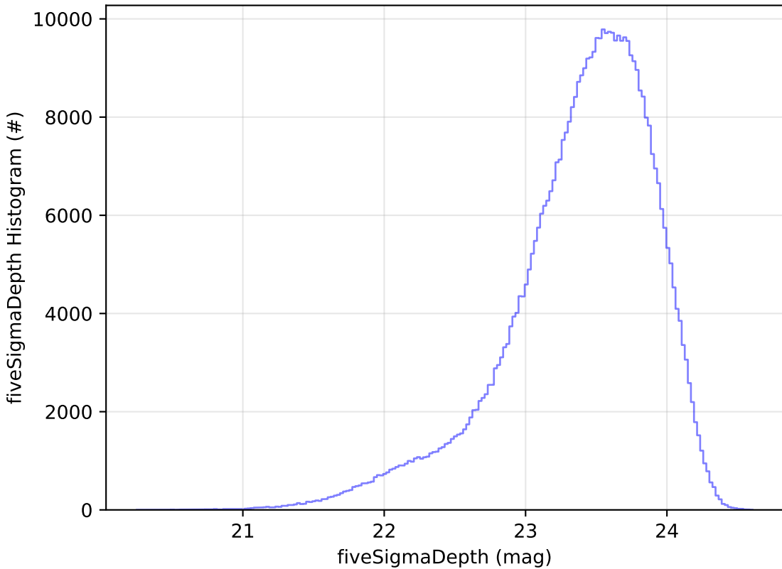
octo_v3.4_10yrs i: fiveSigmaDepth Histogram
