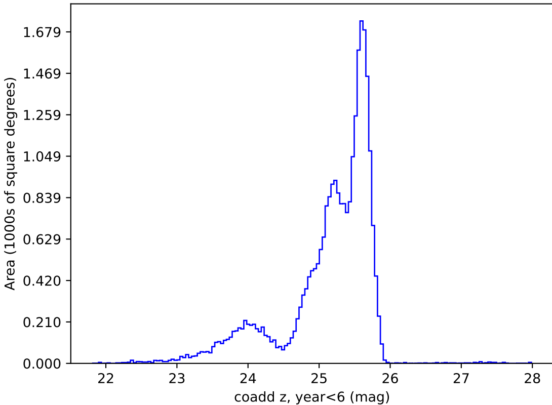
octo_v3.4_10yrs night<2191 and z: coadd z, year<6
