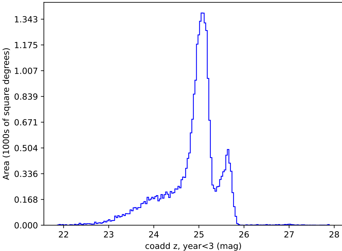
octo_v3.4_10yrs night<1095 and z: coadd z, year<3
