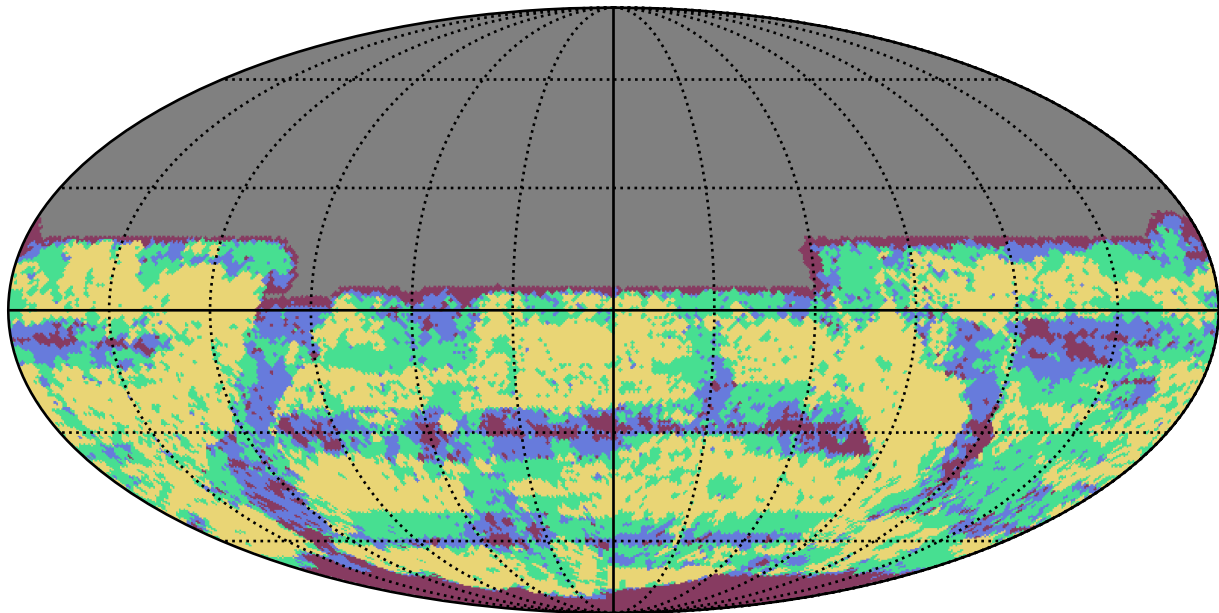
octo_v3.4_10yrs y band: YearCoverage night
