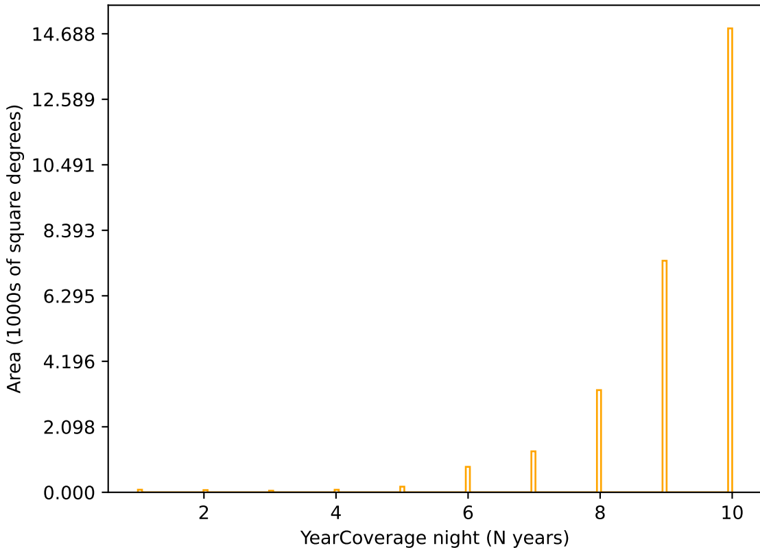
octo_v3.4_10yrs r band: YearCoverage night
