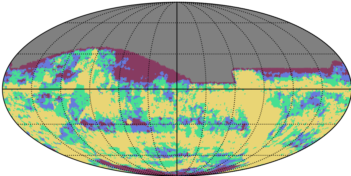
octo_v3.4_10yrs i band: YearCoverage night
