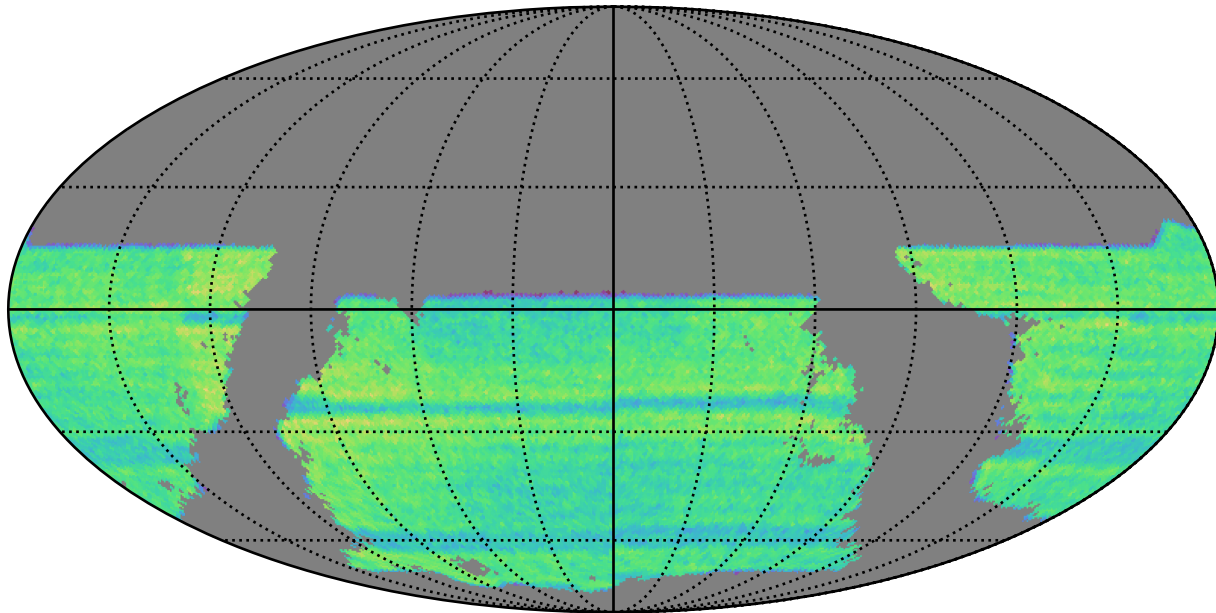
octo_v3.4_10yrs gri band non-DD: WeakLensingNvisits_riz_year8
