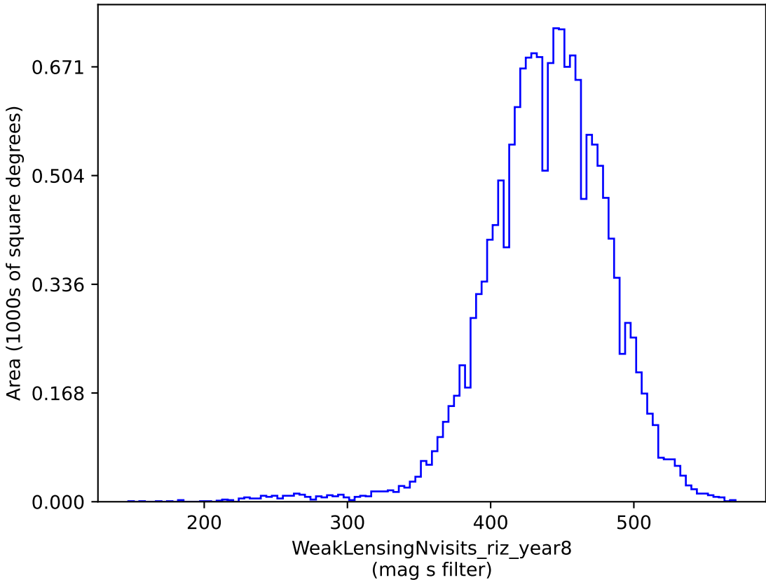
octo_v3.4_10yrs gri band non-DD: WeakLensingNvisits_riz_year8
