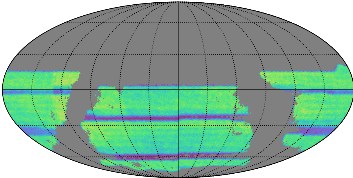
octo_v3.4_10yrs gri band non-DD: WeakLensingNvisits_riz_year7
