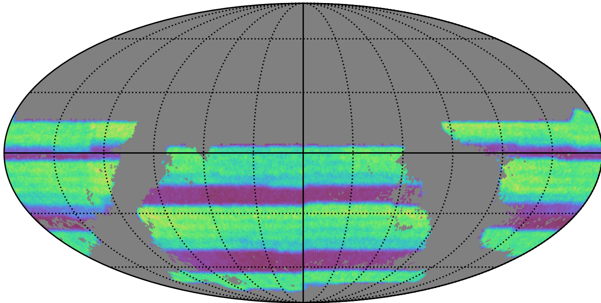
octo_v3.4_10yrs gri band non-DD: WeakLensingNvisits_riz_year6
