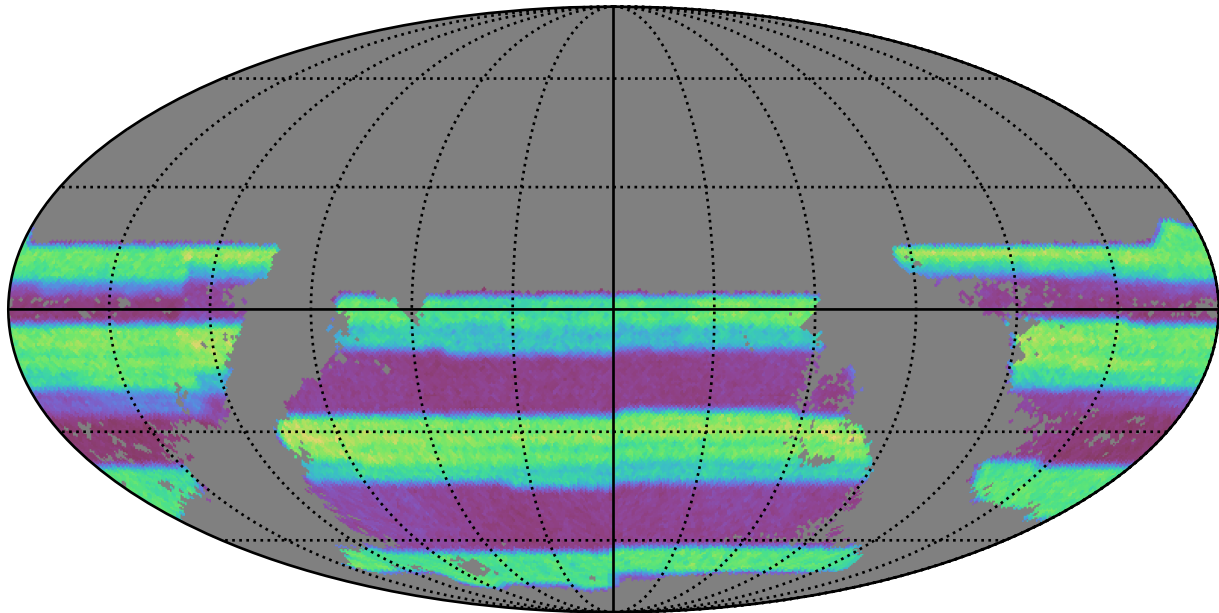
octo_v3.4_10yrs gri band non-DD: WeakLensingNvisits_riz_year5
