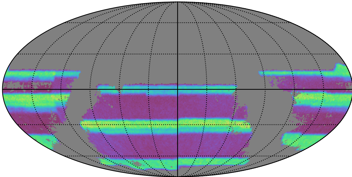
octo_v3.4_10yrs gri band non-DD: WeakLensingNvisits_riz_year4
