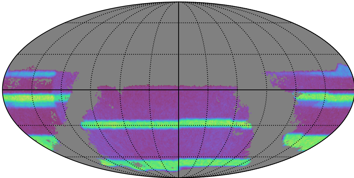
octo_v3.4_10yrs gri band non-DD: WeakLensingNvisits_riz_year3
