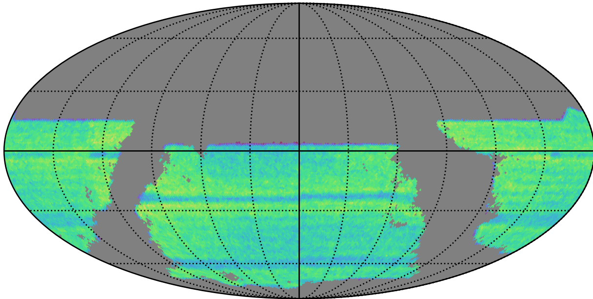
octo_v3.4_10yrs gri band non-DD: WeakLensingNvisits_gri_year8
