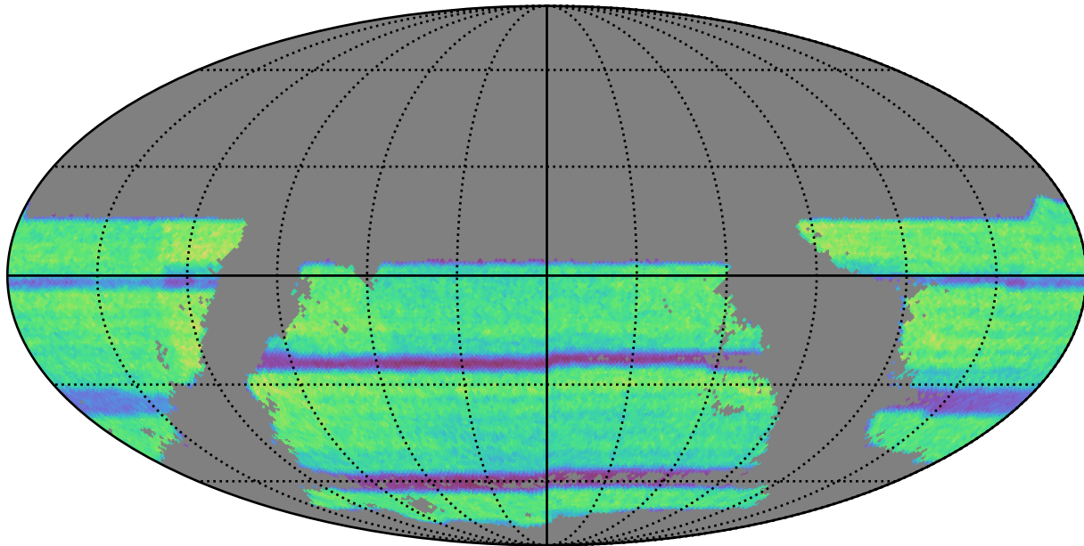
octo_v3.4_10yrs gri band non-DD: WeakLensingNvisits_gri_year7
