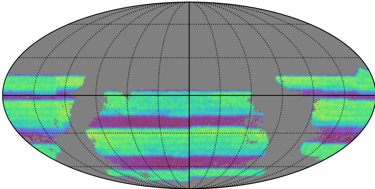
octo_v3.4_10yrs gri band non-DD: WeakLensingNvisits_gri_year6
