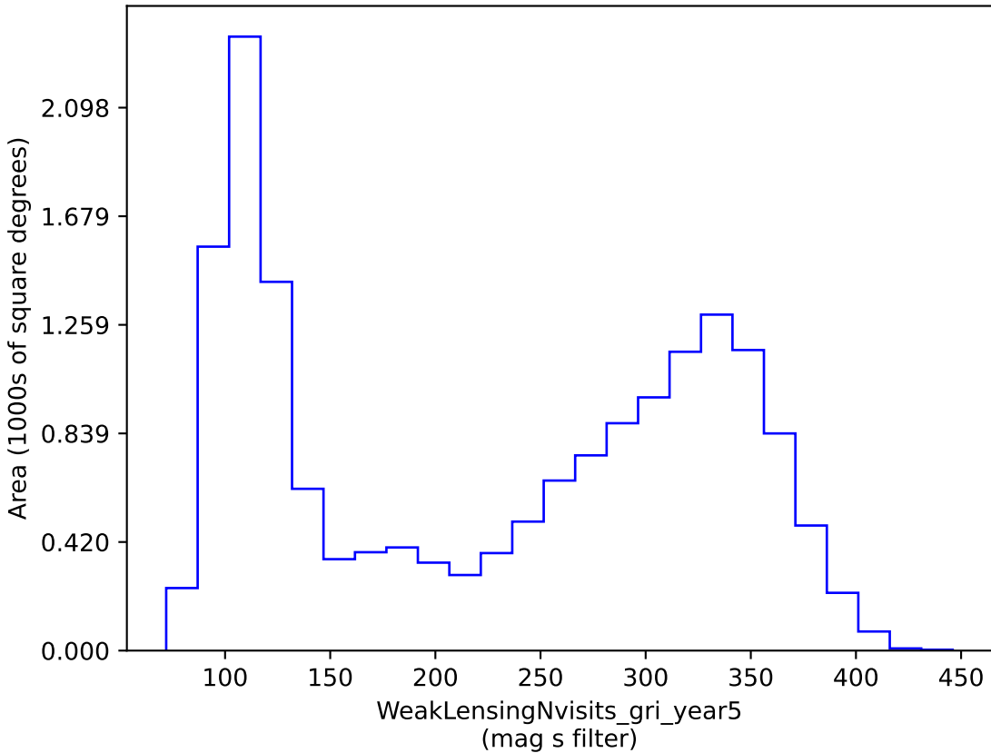
octo_v3.4_10yrs gri band non-DD: WeakLensingNvisits_gri_year5
