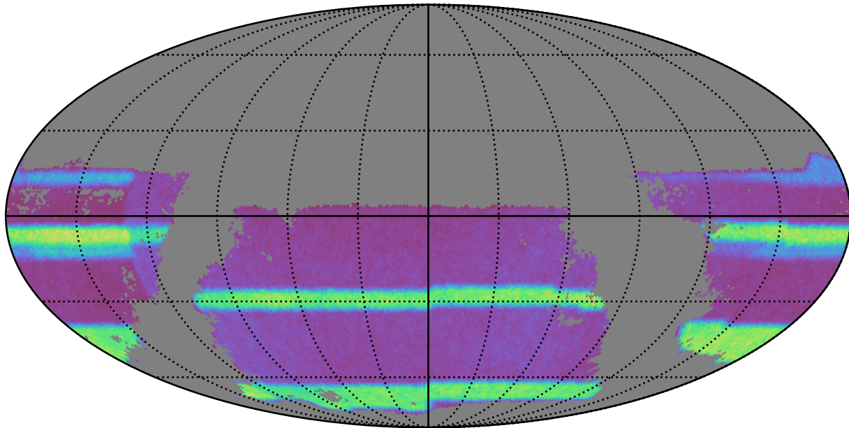
octo_v3.4_10yrs gri band non-DD: WeakLensingNvisits_gri_year3
